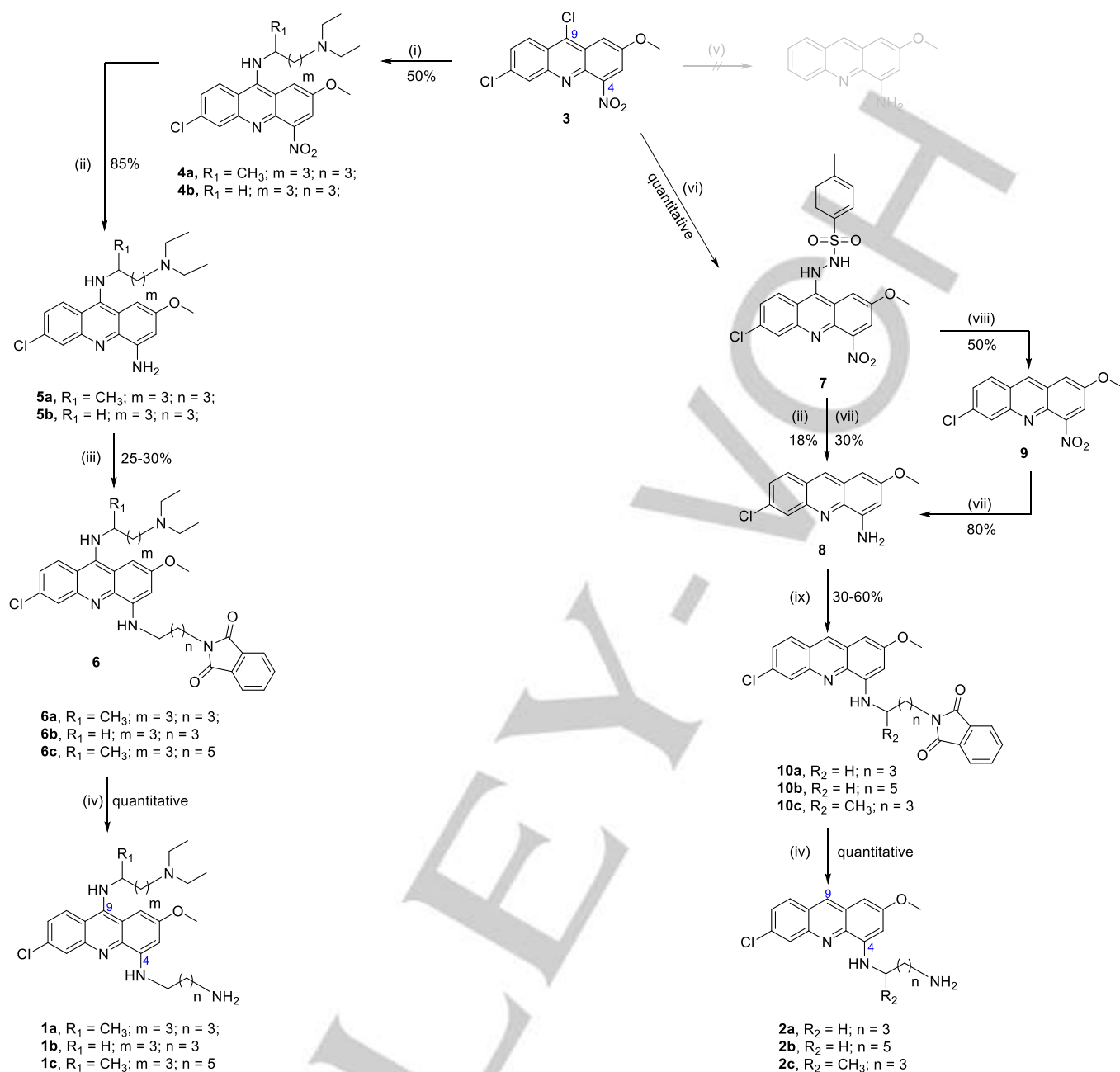
Scheme 1. Synthetic routes towards 4,9-diaminoacridines 1 and 4-aminoacridines 2 . Reagents and conditions: (i) phenol (15 equiv.), Cs 2 CO 3 (1 equiv.), anhydrous DMSO, 4 Å molecular sieves, 100 °C, 2 h, then diamine (4 equiv.), 100 °C, 4 h; (ii) SnCl 2 (5 equiv.), 37% aq. HCl, 0–40 °C, 30 min; (iii) N -( n -bromoalkyl)phthalimide (3 equiv.), CH 3 COONa (3 equiv.), CH 3 CH 2 OH, microwave (MW) heating (100 W, 120 °C) in a pressurized vial (100 psi), 2.5 h; (iv) hydrazine monohydrate (40 equiv.), tetrahydrofuran (THF), 60 °C, 72 h; (v) H 2 (50 psi), Pd/C, CH 3 OH, rt, 5 h; (vi) p -TSH (1 equiv.), CHCl 3 , rt, 24 h; (vii) hydrazine monohydrate (10 equiv.), Pd/C (10% wt), CH 3 OH, 80 °C, 1 h – 3 h; (viii) ethylene glycol/H 2 O (3:1), Na 2 CO 3 (0.0625 M), 95 °C, 1.5 h; (ix) N -( n -bromoalkyl)phthalimide (3 equiv.), Et 3 N (3 equiv.), CH 3 CH 2 OH, MW heating (100 W, 120 °C) in a pressurized vial (100 psi), 3 h.
