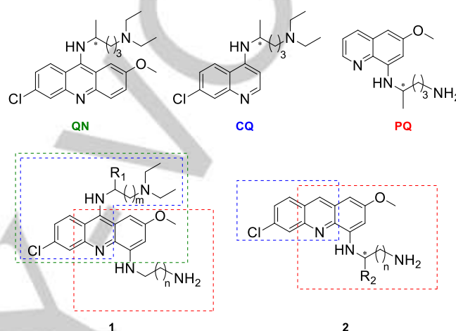
Figure 1. Structures of antimalarials quinacrine (QN) chloroquine (CQ), and primaquine (PQ) – top row; and of 4,9-diaminoacridines (1) and 4-aminoacridines (2) in this work – bottom row.
